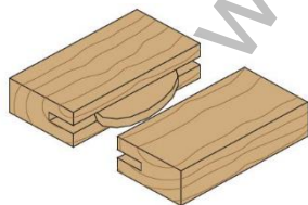
Biscuit joint using bit #7/8/911.040.11
